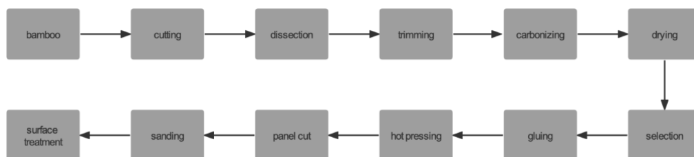
Figure1 Holse & Wibroe traditional bamboo manufacturing process
